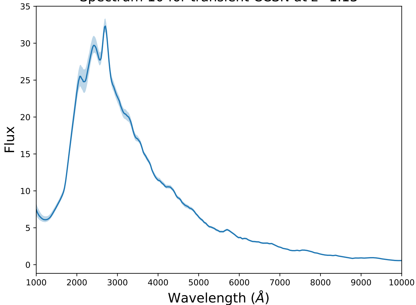
Spectrum 10 for transient CCSN at z=1.13
